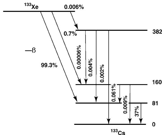
Figure 254. Decay Scheme.
