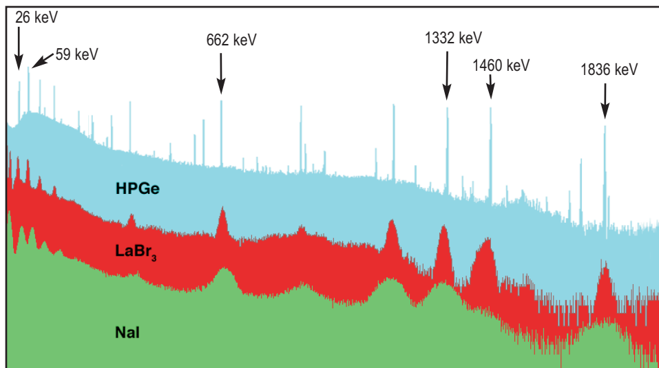
Figure 1. Comparison for \text{LaBr}_3(\text{Ce}) , NaI(Tl), and HPGe spectra.
