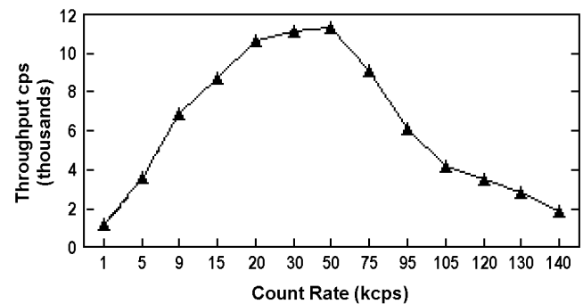
Figure 90. An Example of the Tradeoff Between Throughput and Count Rate.
