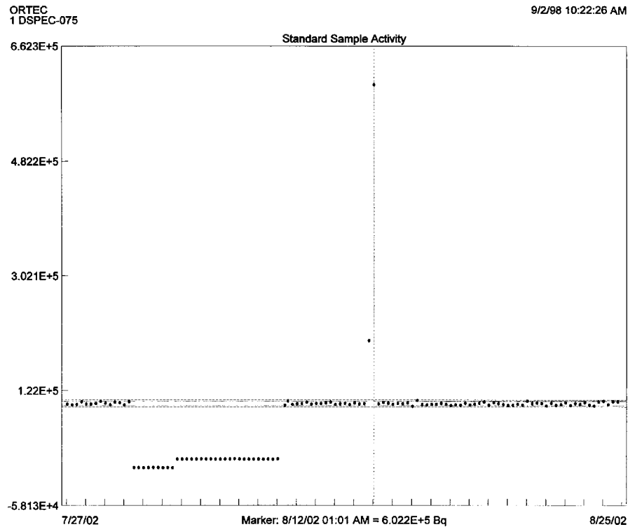
Figure 298. Printout of Control Chart with Fixed Vertical Scale Off.
